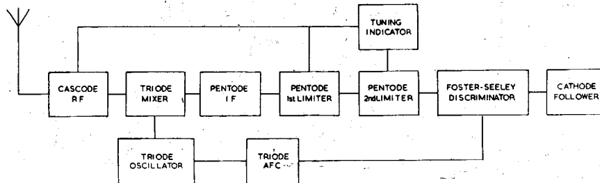
BLOCK CIRCUIT DIAGRAM OF 'TROUGH-LINE 3' F.M. TUNER
